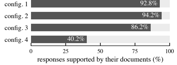
Figure 1: Why the source predicts the label. Adherence rate in the four pooled RAGBench configurations (500 rows each). Scoring each row by its configuration’s rate alone reaches AUC 0.811; the best per-query score reaches 0.637 and the headline 0.843.
