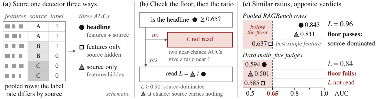
Figure 2: Three numbers and a precondition. (a) Schematic: one detector is scored three ways, given features plus source (the headline, circle), features only (square), and source only (triangle). (b) The ratio L of the source-only AUC to the headline is read only if the headline passes the floor. (c) Two panels with similar L get opposite verdicts, because only one passes the floor (on RAGBench the square is the best single feature).
