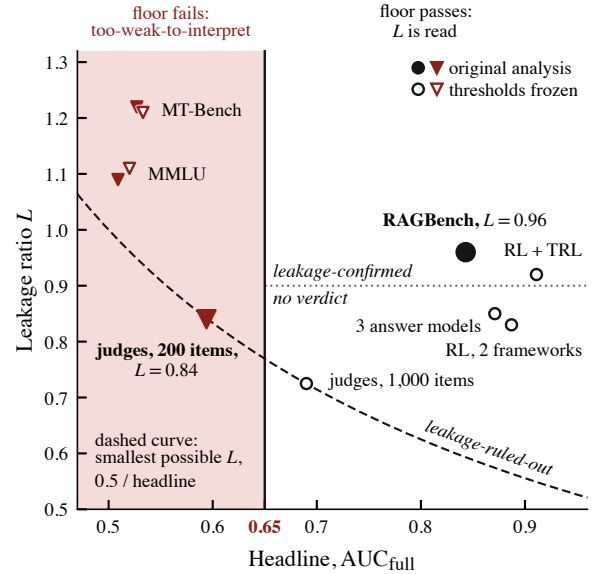
Figure 3: Leakage ratio L against the headline AUC_{full} for the ten audits of Table 1. High L occurs on both sides of the floor: horizontal position, not height, decides whether L is read. Triangles fail the floor and circles pass it; hollow marks were audited with both thresholds frozen (for MT-Bench and MMLU, the second feature set). The dotted line is the band, L \geq 0.90 . No audit can lie below the dashed curve, and the two crossed judge panels lie on it.
