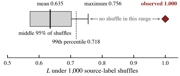
Figure 4: No source-label shuffle reaches the observed L = 1.000 (maximum 0.756). The null is for the unfiltered RL panel ( n = 117 ; 1,000 shuffles of the source label, with features and fault labels held fixed). The box spans the middle 95% of shuffles; ticks mark the stored mean (0.635), 99th percentile (0.718), and maximum (0.756); the diamond is the observed L = 1.000 . Per-shuffle values were not stored, so the figure shows the stored summary. Only the direction of the separation is interpretable, because the source label restates fault status in this panel.
